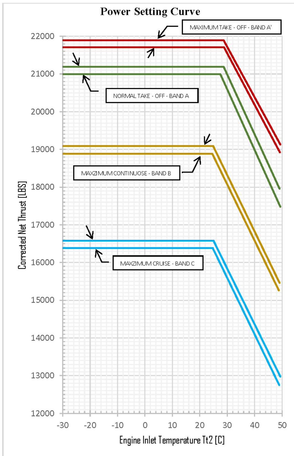
Figure 9-1: Power Setting Curve (4)
