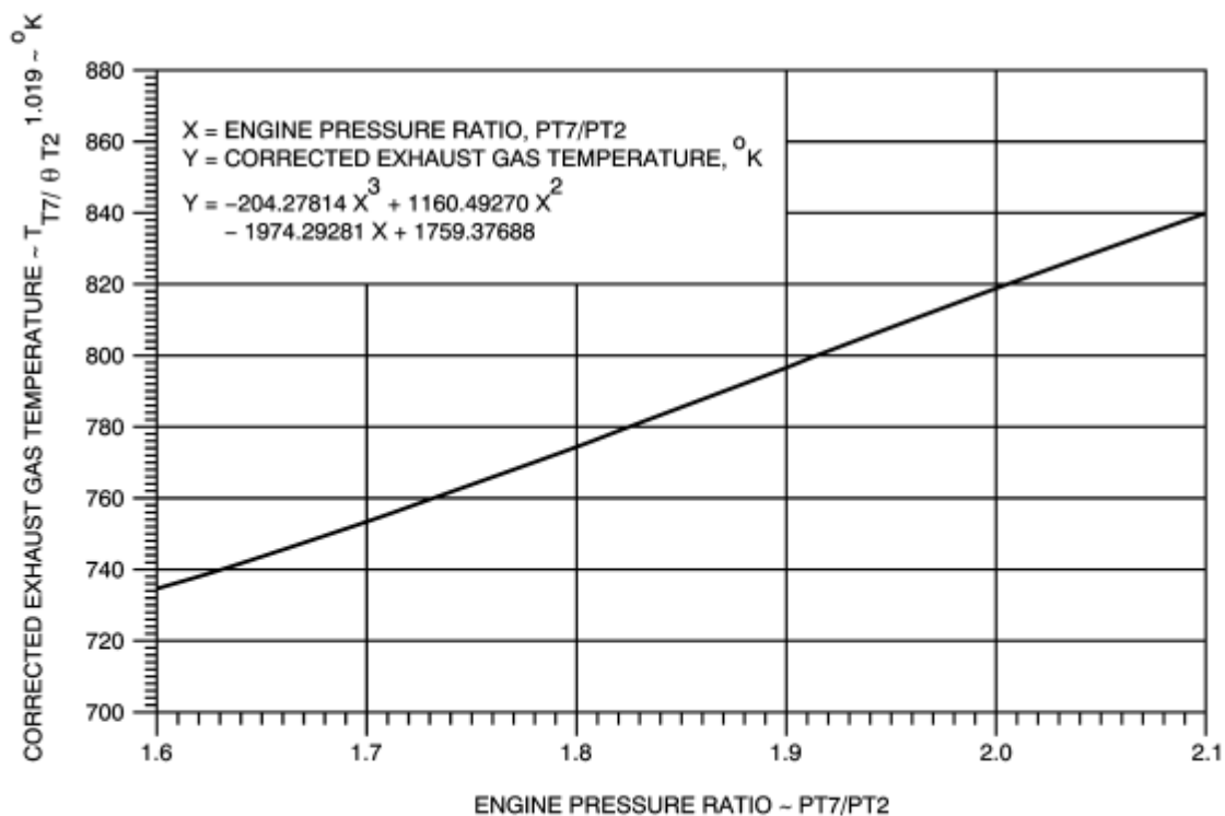
Figure 7: EGT Margin Check Curve (Figure 1313, Testing-06)
