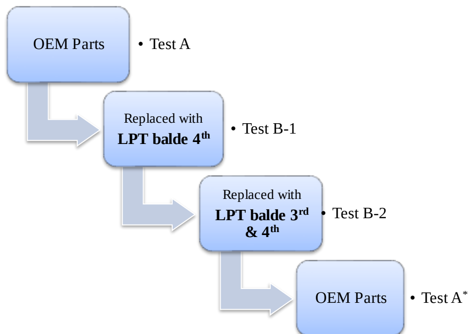
Figure 5-1: Back-to-back test procedure
