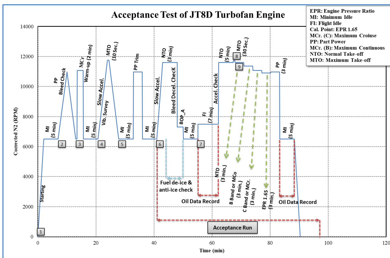
Figure 5-2: Procedure of step4 of Test B/ Acceptance test
