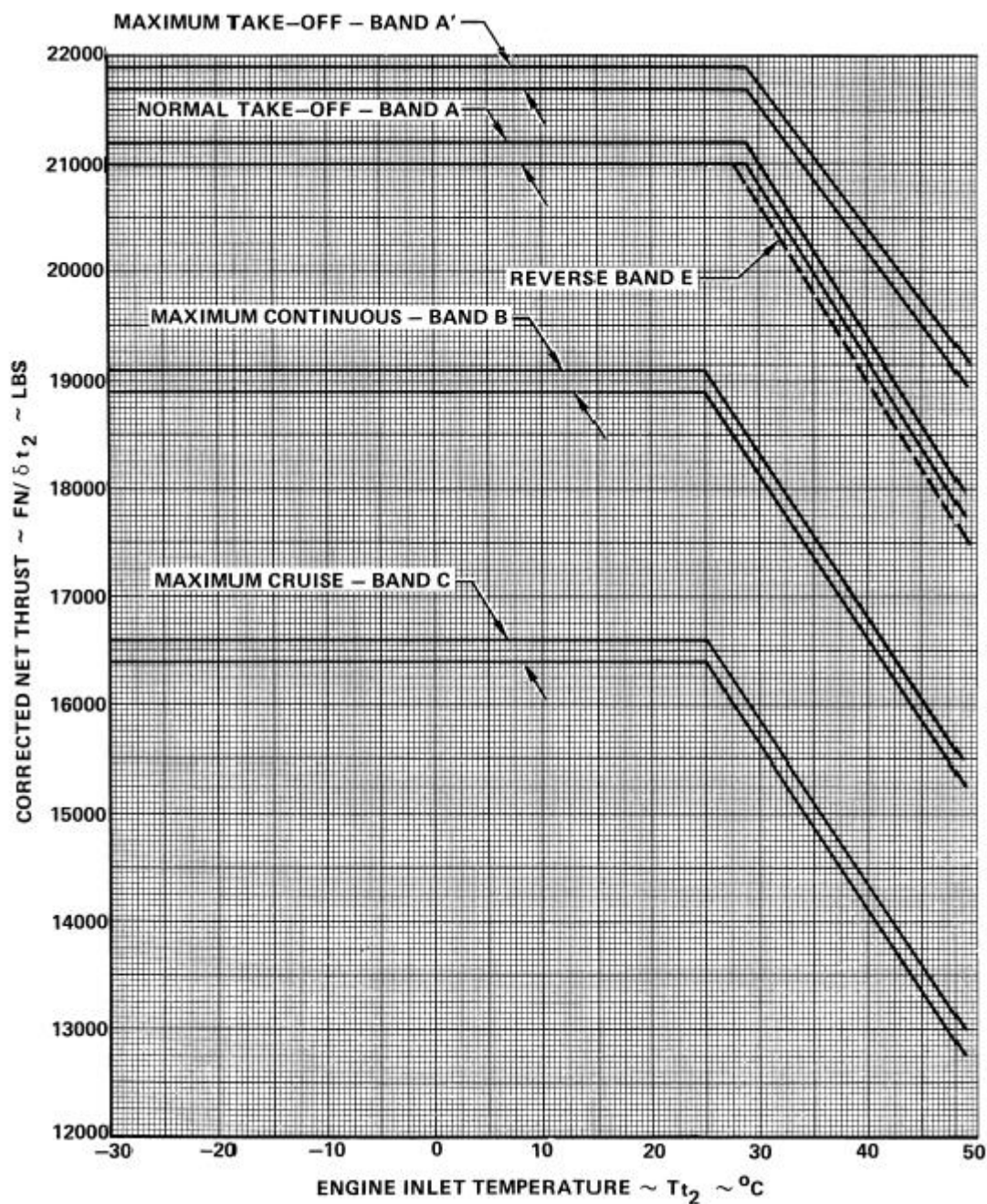
Figure 3: Power Setting Curve (Figure 1304, Testing-06)
