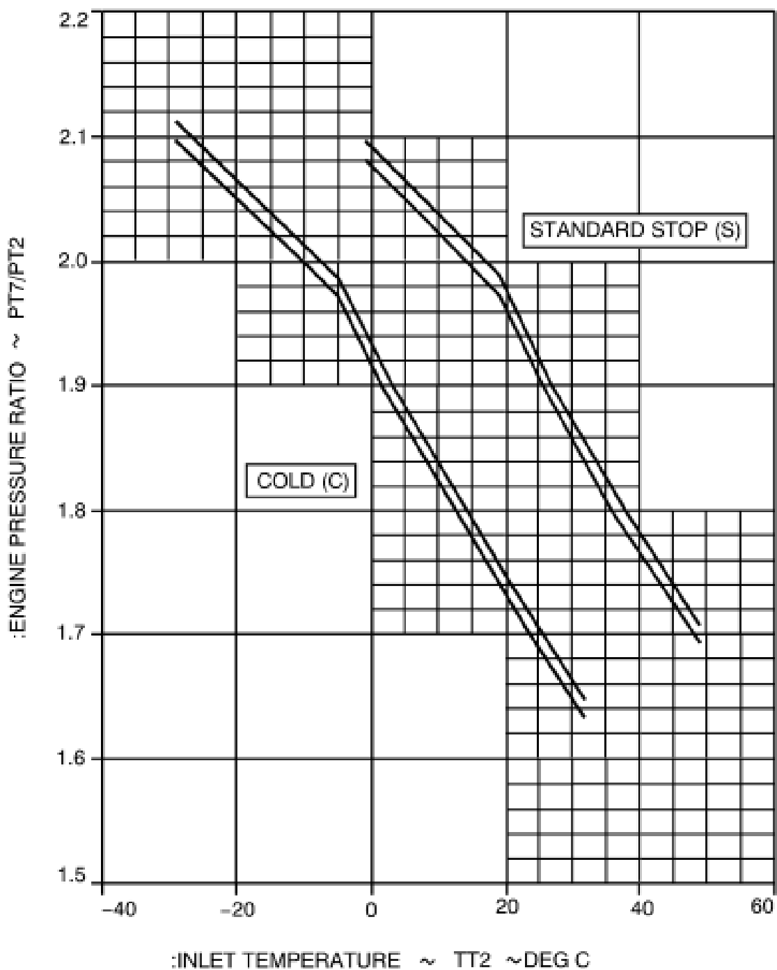
Figure 5: Part Power Trim Curve (Figure 1309, Testing-06)
