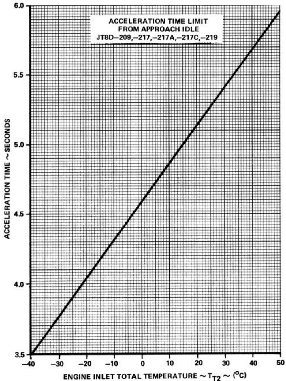
Figure 6: Acceleration Time Limit From Approach Idle (Figure 1306, Testing-06)
